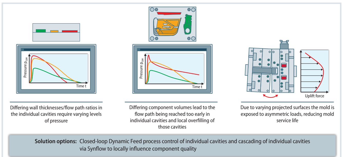
Fig. 3. Challenges in designing family molds.. © Synventive
